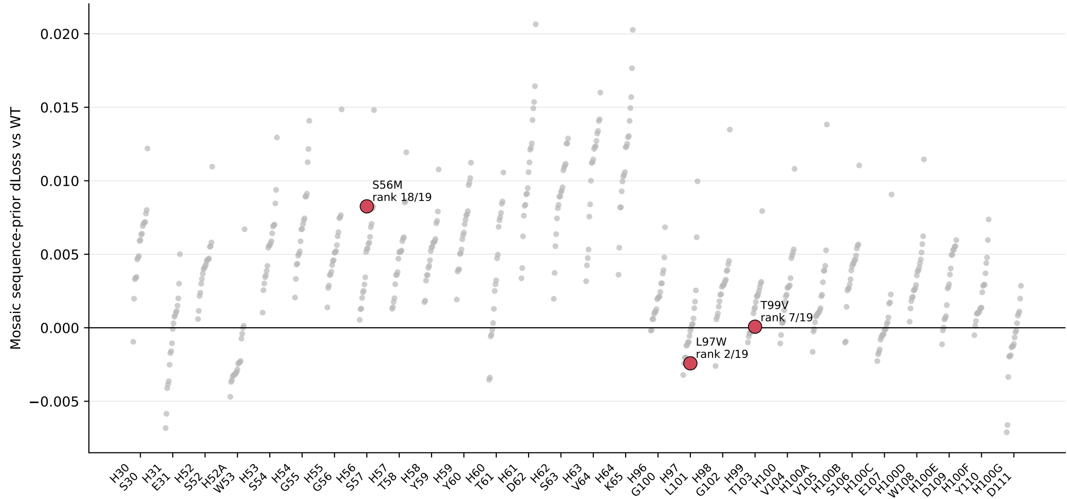
VHH72 CDR single-substitution loss distribution by site
